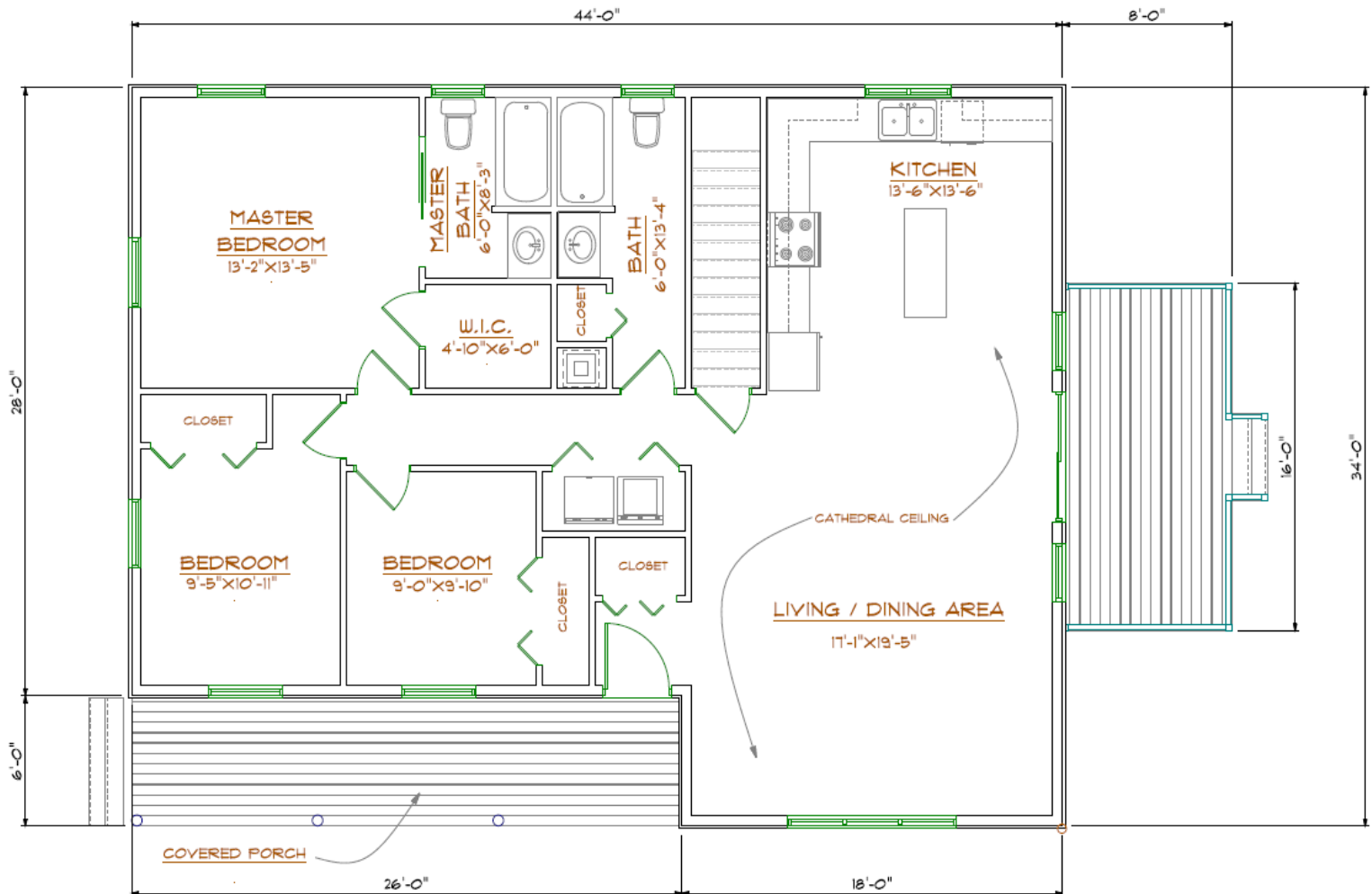
Rangeley Main Floor Plan 1340 Sq. Ft.
