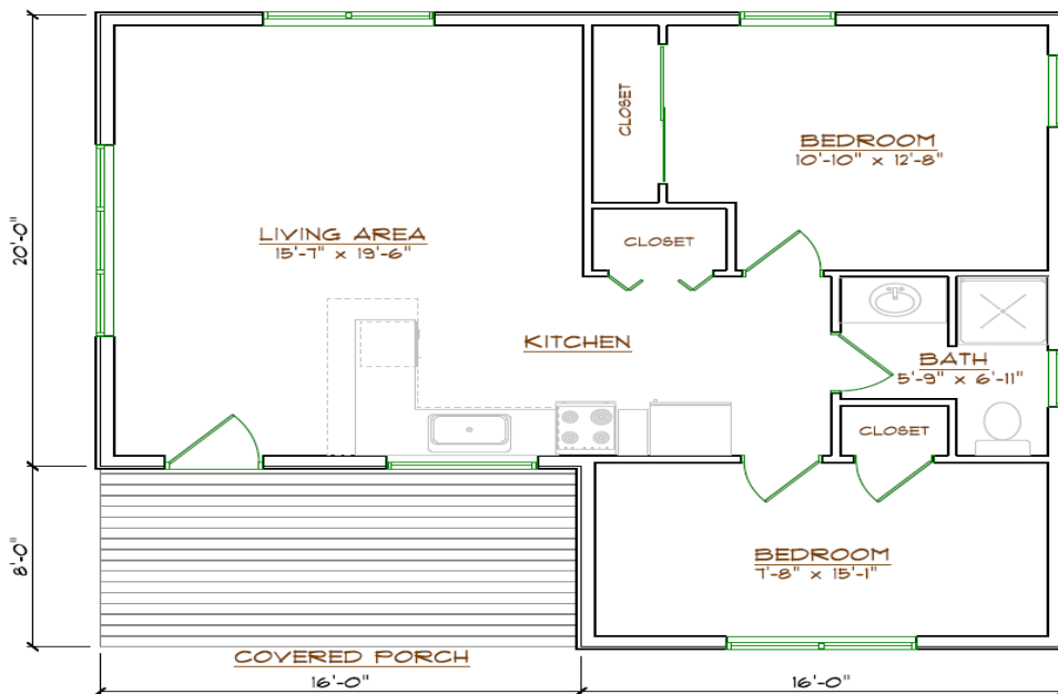
The Kennebago 2 Main Floor Plan 768 Sq. Ft.
