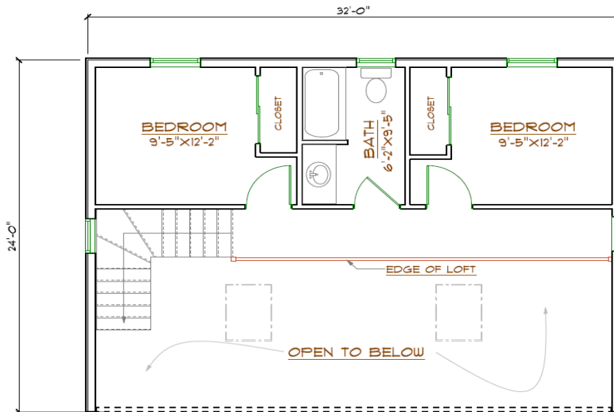
The Gunstock Upper Floor Plan 414 Sq. Ft.
