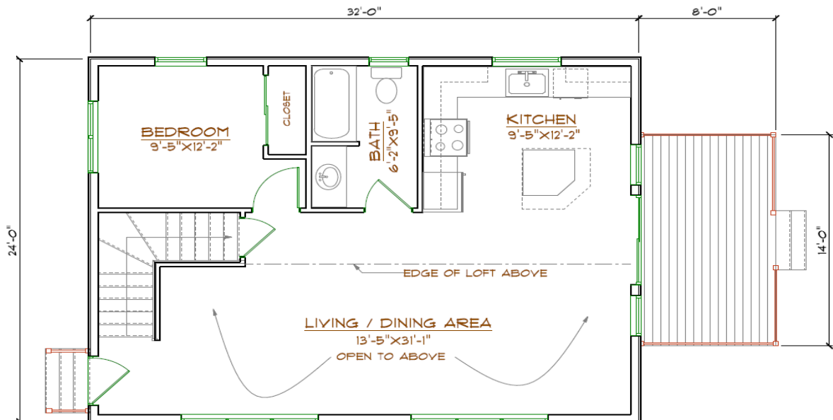
The Gunstock Main Floor Plan 768 Sq. Ft.
